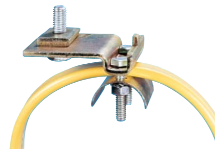
6 CABLE/HOSE CLAMP
