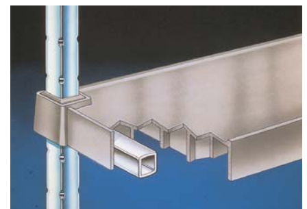
Plasteel® Cutaway
