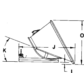
ROCKER AND STOP FOR LH HOPPERS
