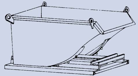
No. 10 CRANE PICK-UP EYES (2 EACH SIDE) 8 LBS.
