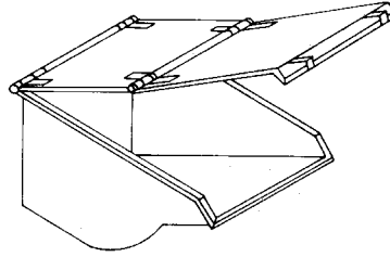
TYPE B DOUBLE HINGED – BACK AND CENTER
