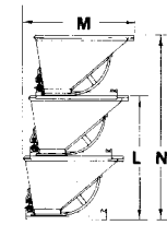
LH-50 & LH-100 Hoppers Stack Only*
